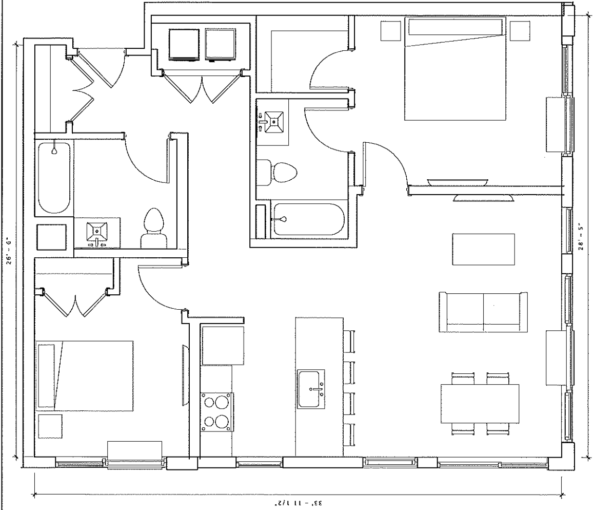
UNIT TYPE 'D2' PLAN
